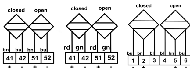
wiring diagram: left general, centre SJ 3,5-S1N and right NJ3-18GK-S1N
