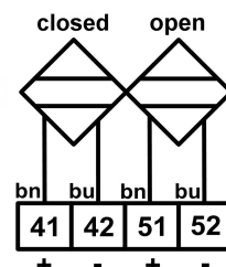
wiring diagram
