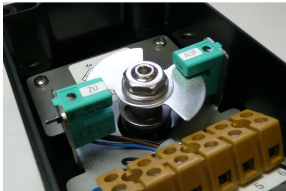
image: inner view Pepperl+Fuchs sensors SB 3,5-E2 with adjustable switching cams
